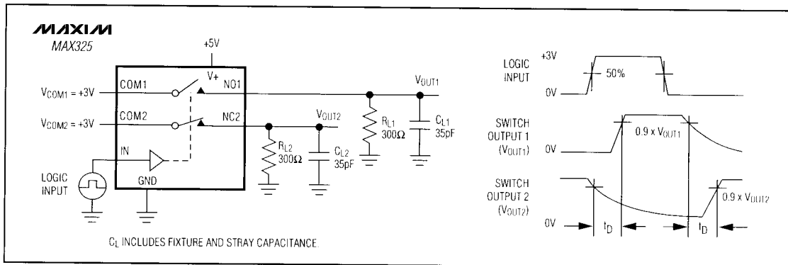
Figure 3. Break-Before-Make Interval (MAX325 only)
