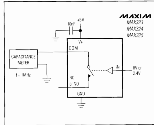
Figure 8. Channel-On Capacitance
