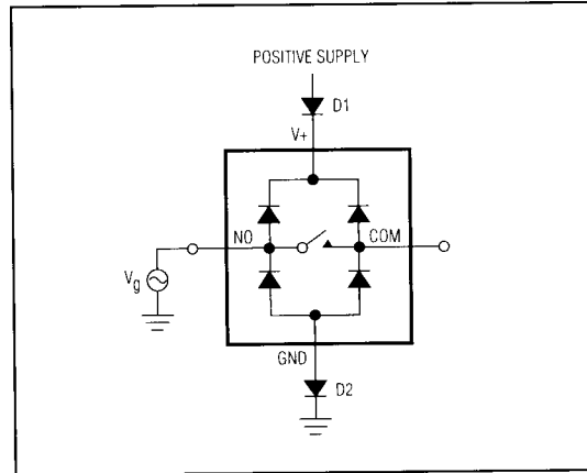
Figure 1. Overvoltage Protection Using Two External Blocking Diodes
