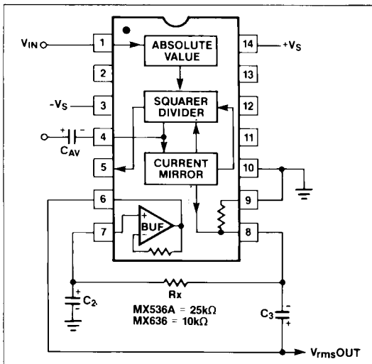
Figure 8. MX536A/MX636 with a 2 Pole Output Filter
